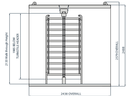
Side view elevation
